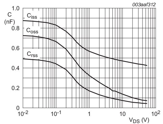
Fig 13. Input, output and reverse transfer capacitances as a function of drain-source voltage; typical values
